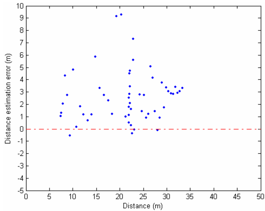
Figure 3.9: Scatter plot of the distance error for Setup 2 at 200 MHz bandwidth.
