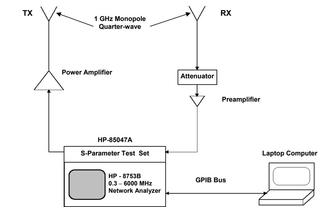
Figure 3.1: Frequency domain measurement system
